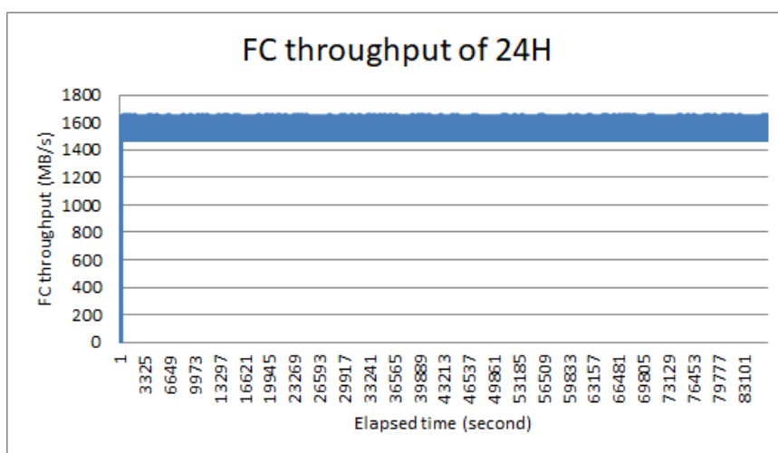
Figure 11: 24-hour Throughput of LTX at FC16G
