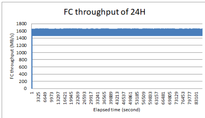
Figure 10: 24-hour Throughput of LDCA at FC16G
